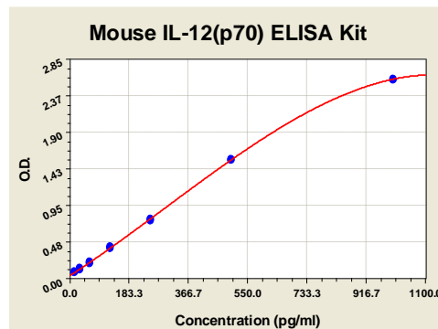
Figure 1: IL-12 (P70) Standard Curve. Using the mouse IL-12 (P70) ELISA Kit, O.D. data was graphed against IL-12 (P70) protein concentration. The TMB reaction was incubated at 37° C for 16 min.
